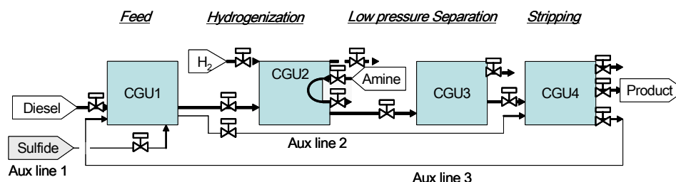
Figure 3. HDS CGU Diagram with Additional Piping System
