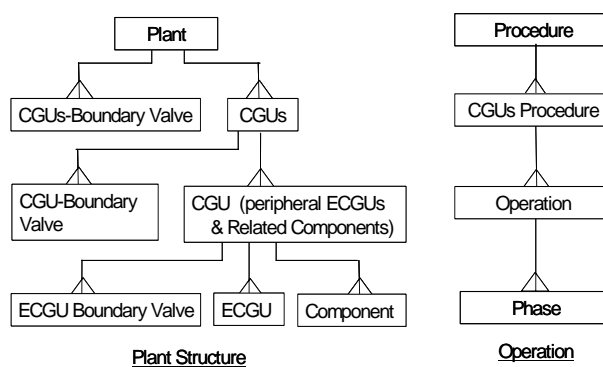
Figure 2 Information models
